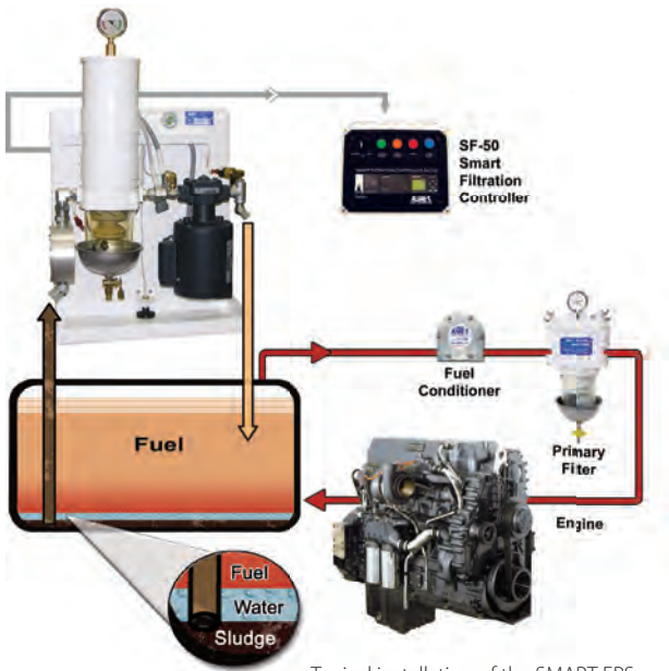
Typical installation of the SMART FPS Fuel Polishing and Transfer System
